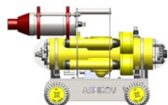
PIPESCANNER (LASER ABOVE WATER OR ACOUSTIC UNDER WATER) Remotely operated wheelskid with pipe profiling sonar or laser scanner
